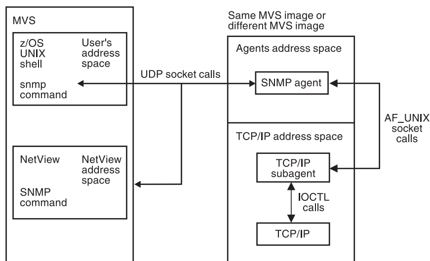
Figure 128. Overview of SNMP support
