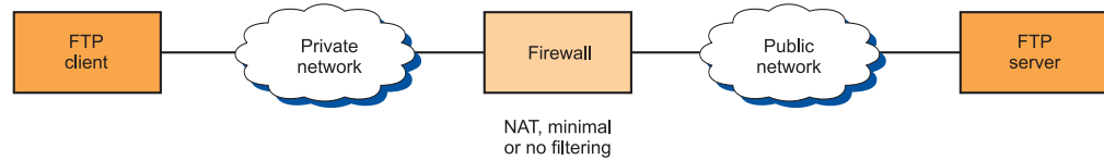
Figure 72. SSL/TLS-secured FTP session scenario 1
