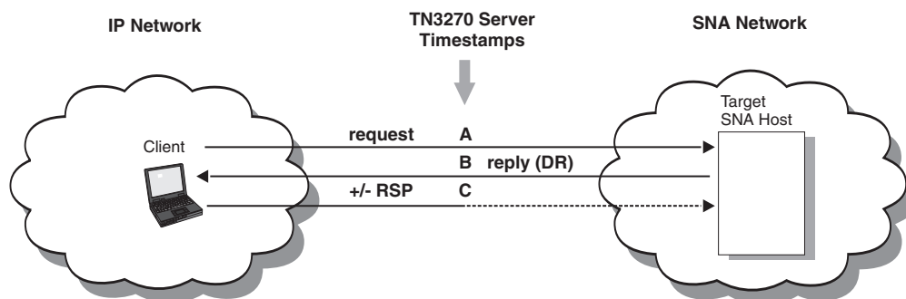
Figure 70. Typical Telnet data flow
