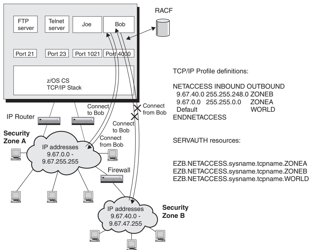
Figure 20. Network access control example
