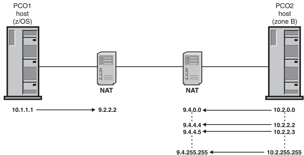
Figure 104. Partner company with NAT model
