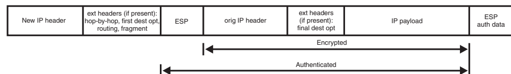
Figure 96. IPv6 packet encapsulated using ESP in tunnel mode
