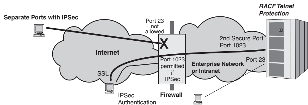
Figure 26. Combining Telnet security with IPSec client-to-firewall authentication
