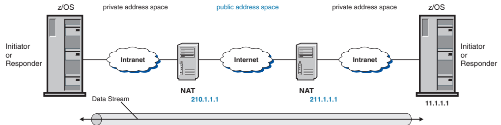
Figure 110. z/OS host to z/OS host, double NAT
