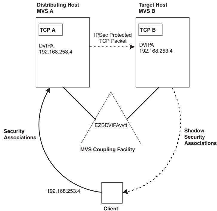
Figure 42. Sysplex distributor with SWSA
