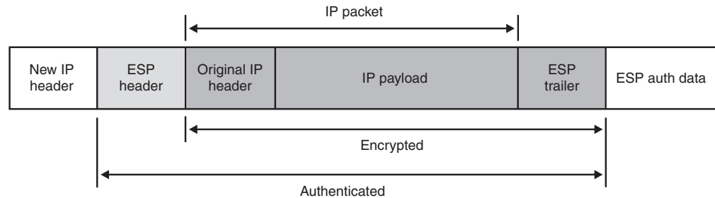
Figure 94. IPv4 packet encapsulated using ESP in tunnel mode
