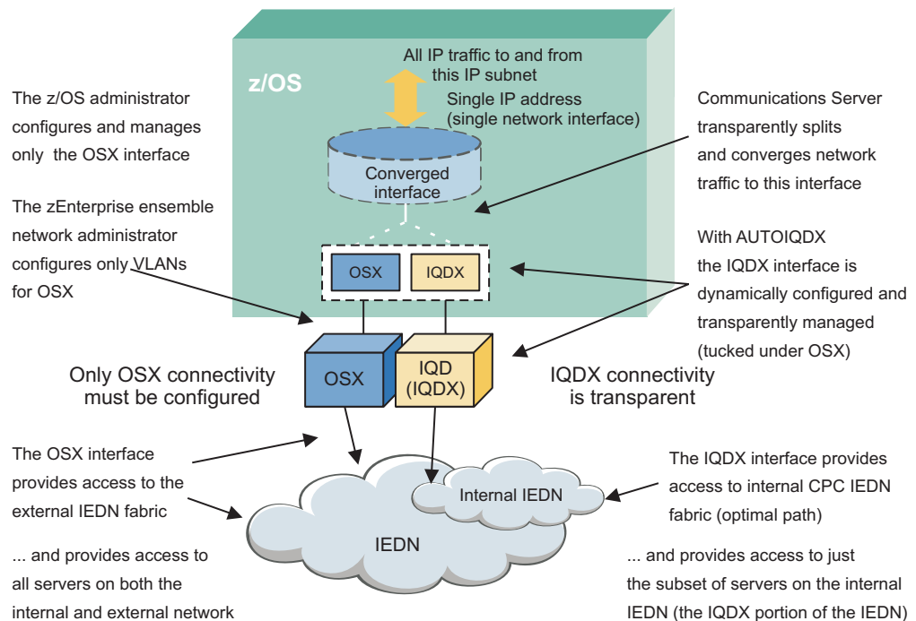
Figure 50. z/OS Communications Server IEDN-enabled HiperSockets overview
