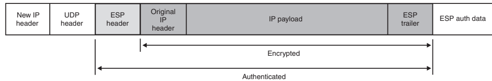
Figure 98. UDP-encapsulated tunnel mode
