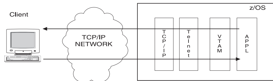
Figure 62. Telnet connectivity
