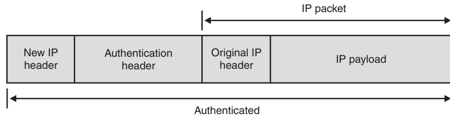
Figure 93. IPv4 packet encapsulated using AH in tunnel mode
