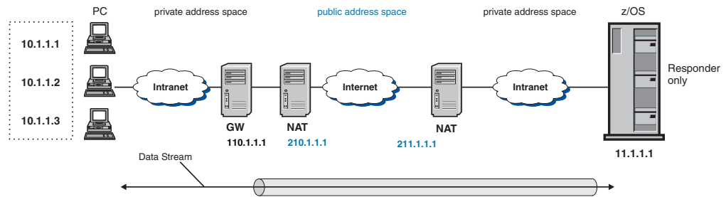
Figure 112. z/OS in a host-to-security gateway configuration
