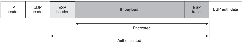
Figure 97. UDP-encapsulated transport mode
