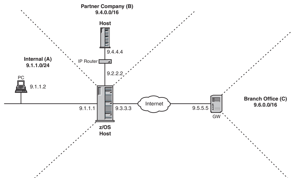
Figure 101. Security model network
