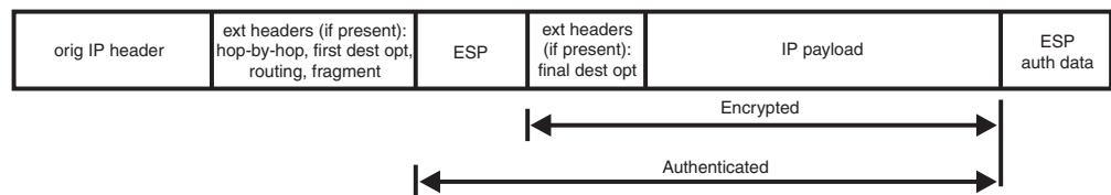
Figure 92. IPv6 packet encapsulated using ESP in transport mode
