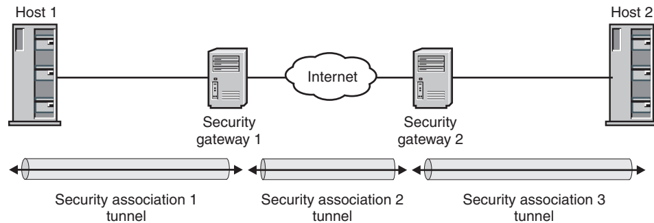
Figure 108. Cascaded tunnels
