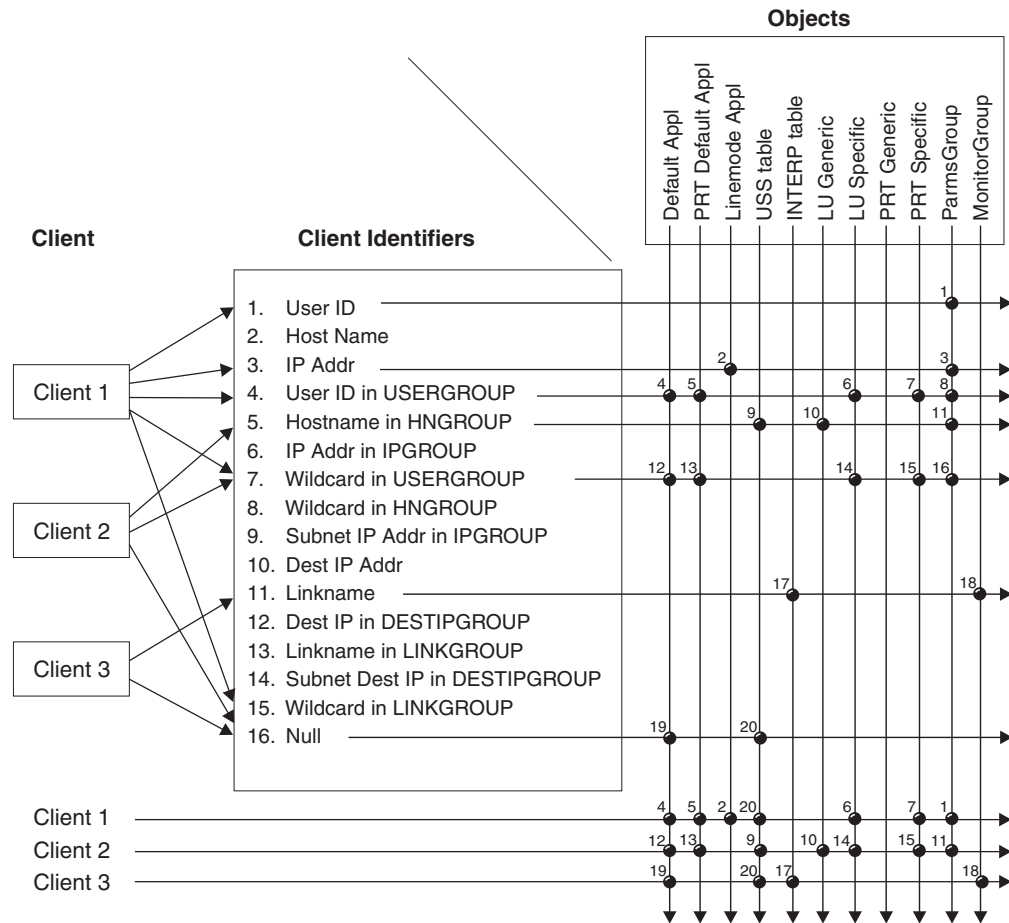
Figure 67. Search method
