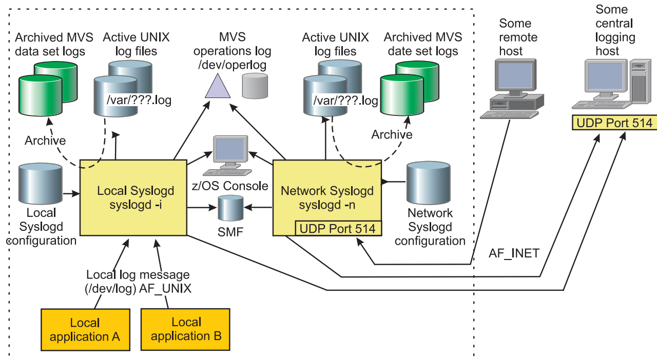
Figure 2. syslogd operation
