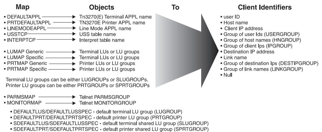
Figure 66. Mapping model
