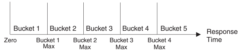
Figure 71. Time buckets
