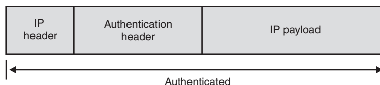
Figure 89. IPv4 packet encapsulated using AH in transport mode
