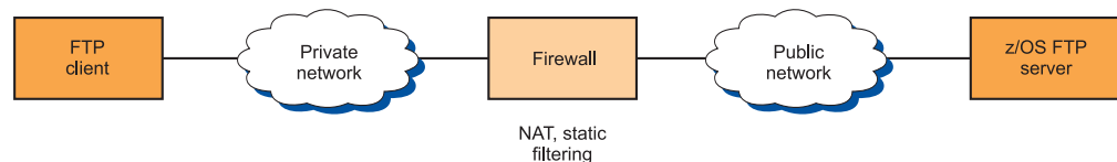
Figure 74. SSL/TLS-secured FTP session scenario 3
