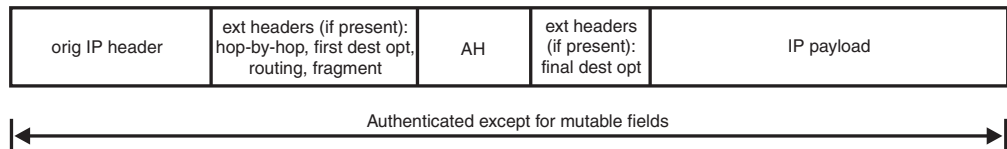
Figure 91. IPv6 packet encapsulated using AH in transport mode
