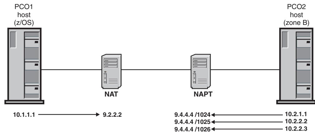
Figure 105. Partner company with NAPT model
