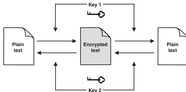
Figure 99. Symmetric encryption
